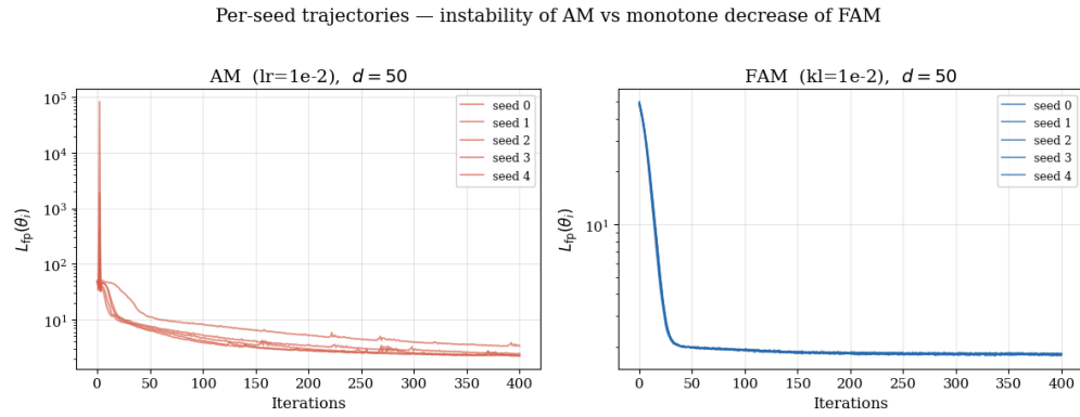
Figure 3: Loss curves for Adjoint Sampling. Left: Adam-only AM exhibits unstable, non-monotonic training. Right: FAM achieves a monotonic decrease in loss.
